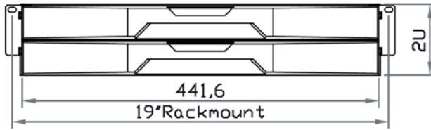
Rear View
