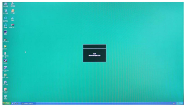
Resolution 1600X 1200
