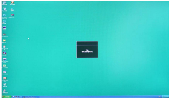
Resolution 1920 x 1080
