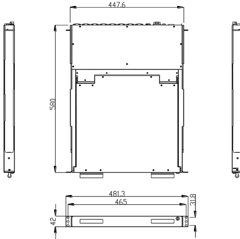
Rear of AVP117WTHB-16e
