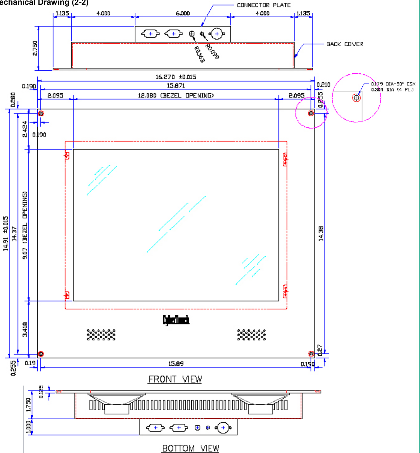
Mechanical Drawing (2-2)
