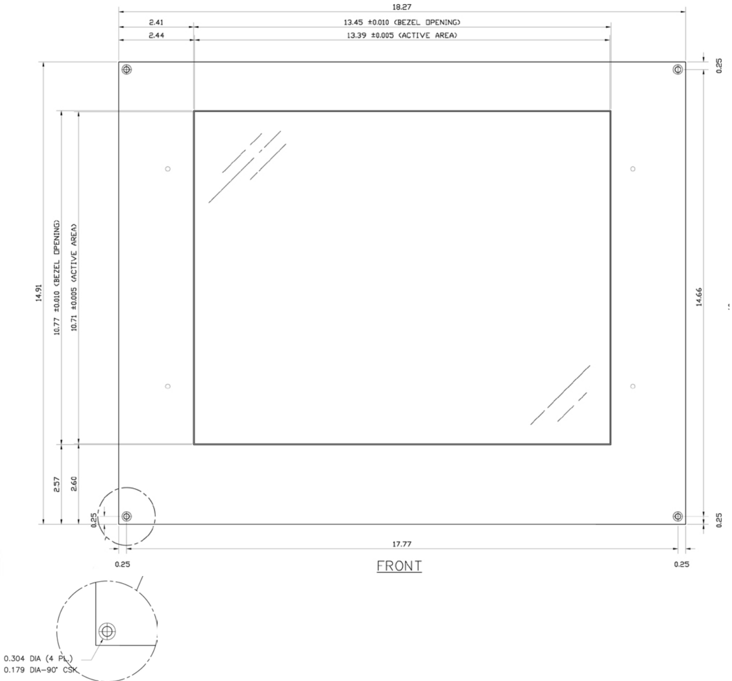
Mechanical Drawing (2-2)
