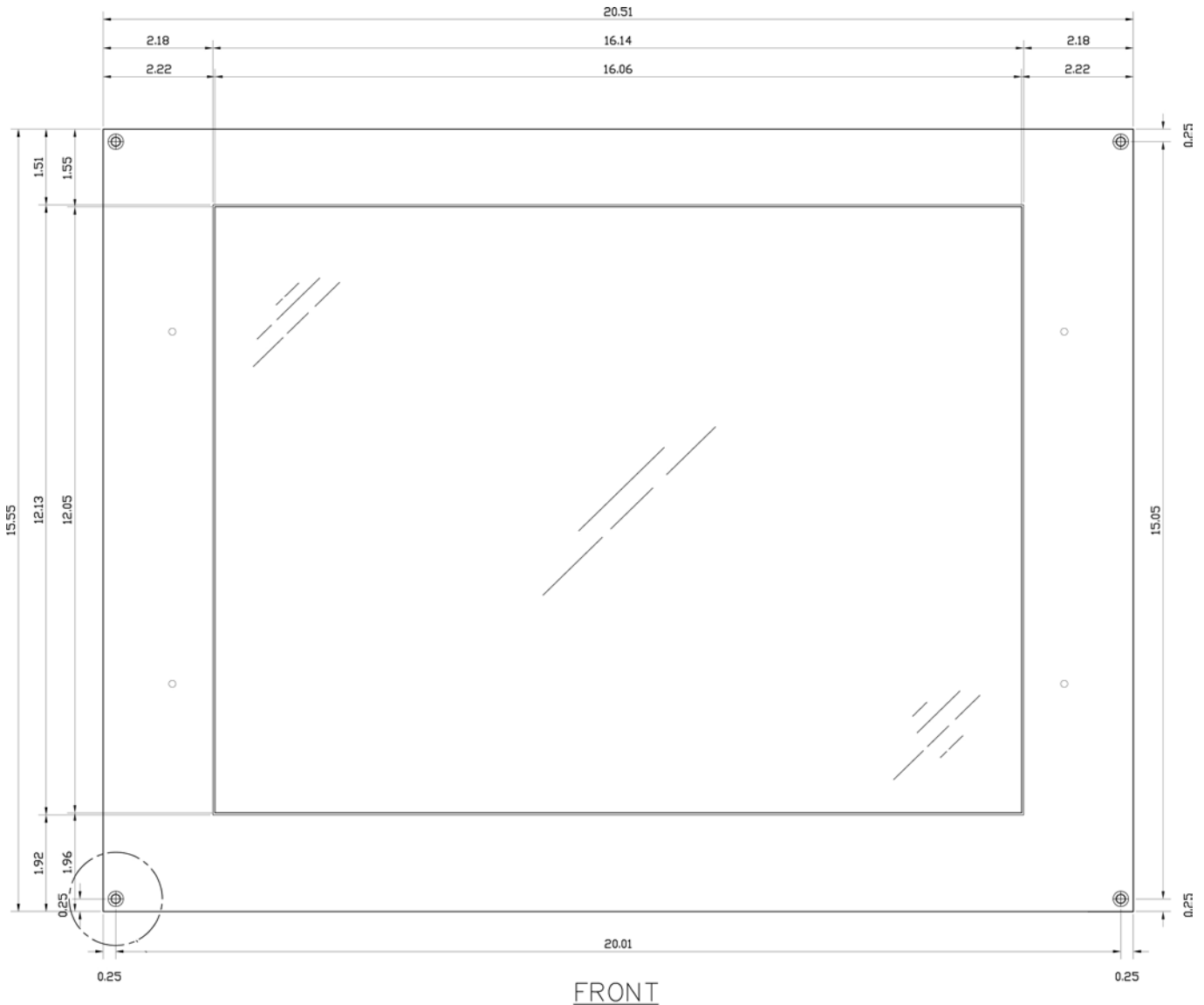
Mechanical Drawing (2-2)
