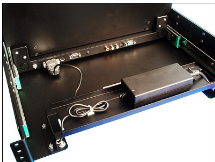
Rack Adaptor with optional power supply and bridge
