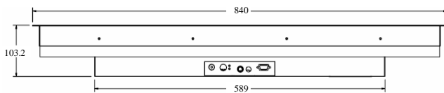
Bottom View
