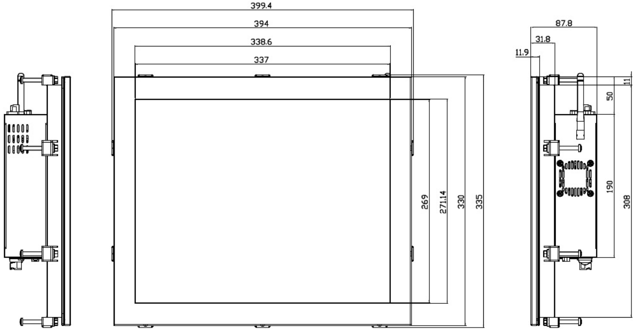
MPC1700CD Drawing
