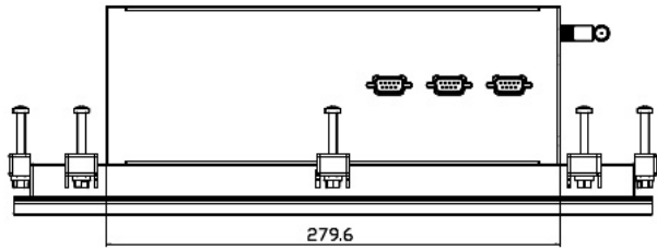
MPC1700CD-PCI Drawing
