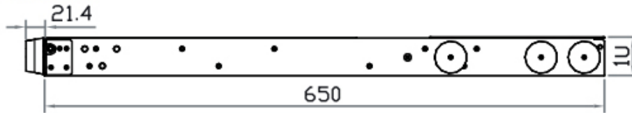
Side View
