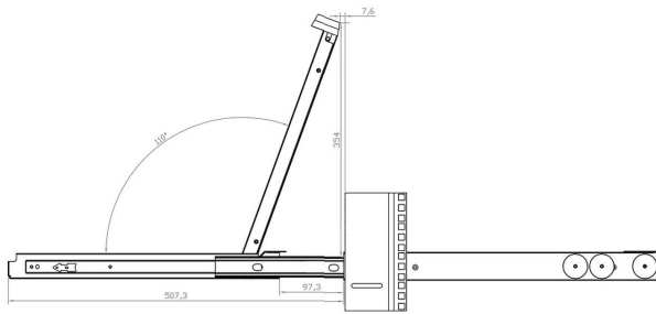
Lockable Railway
