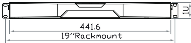
Rear View
