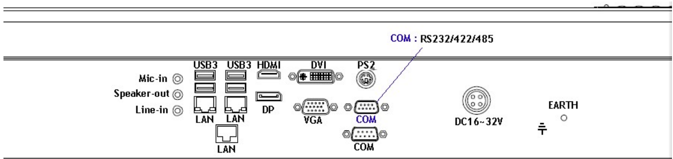
I/O Ports
