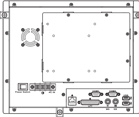
Rear View - with Terminal Block
