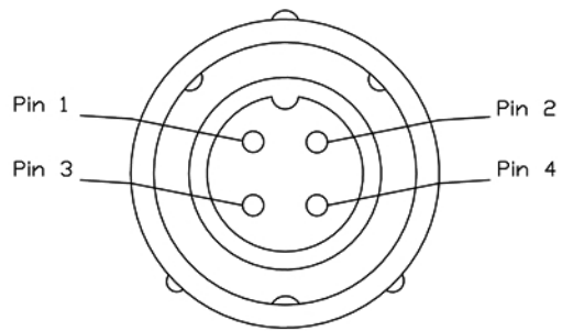
VIEW "A-A"
