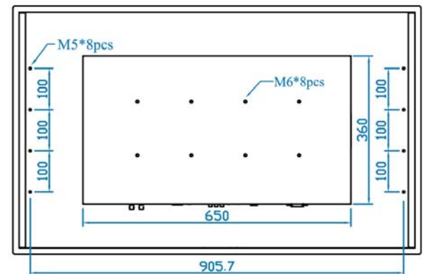
Rear View
