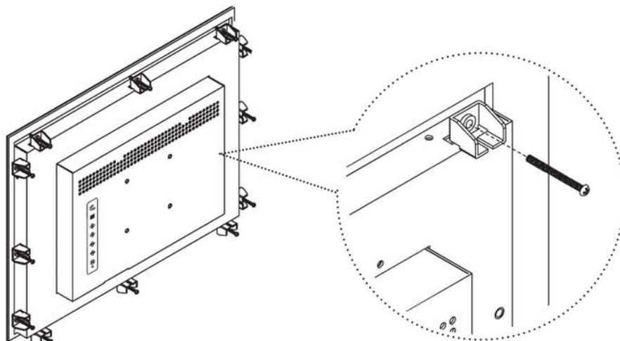
Mounting bracket B
