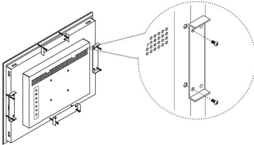
Mounting bracket A
