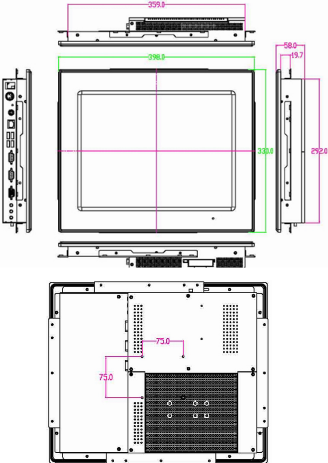
WPC1500 Mechanical Drawing
