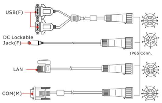
IP65 connector / cable
