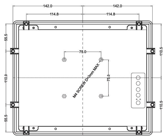
CUT OUT DIMENSION(264x210mm) UNIT:mm
