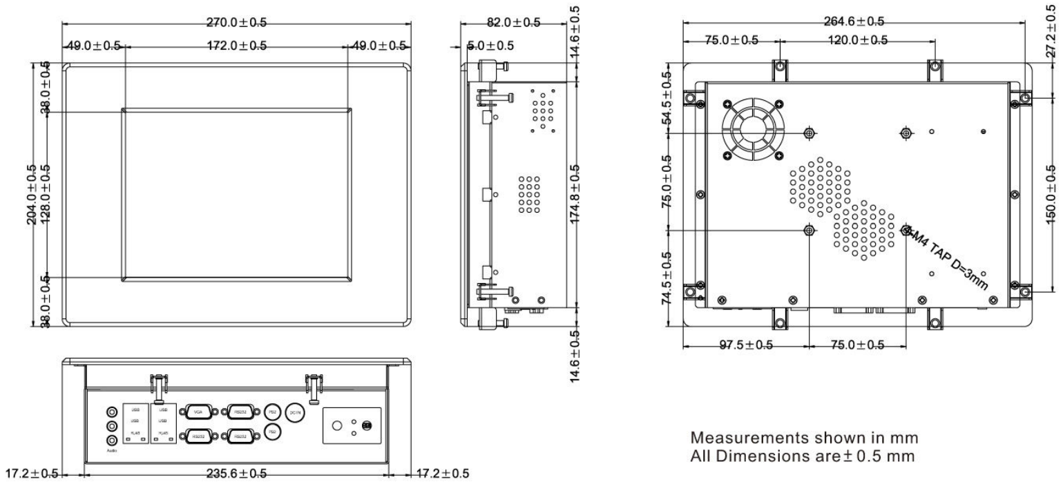
BOTTOM VIEW
