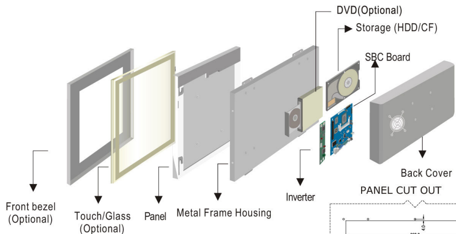
Modularized Construction
