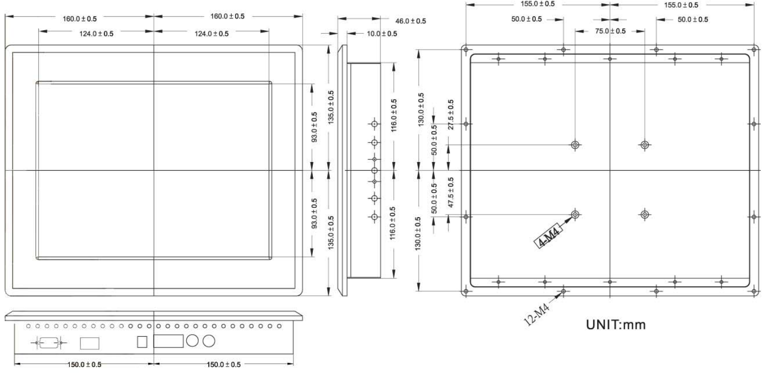
MECHANICAL DRAWING
