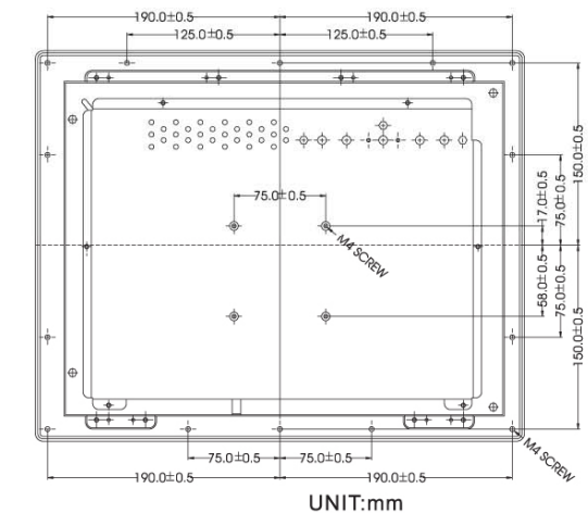
CUT OUT DIMENSION(360x280mm)
