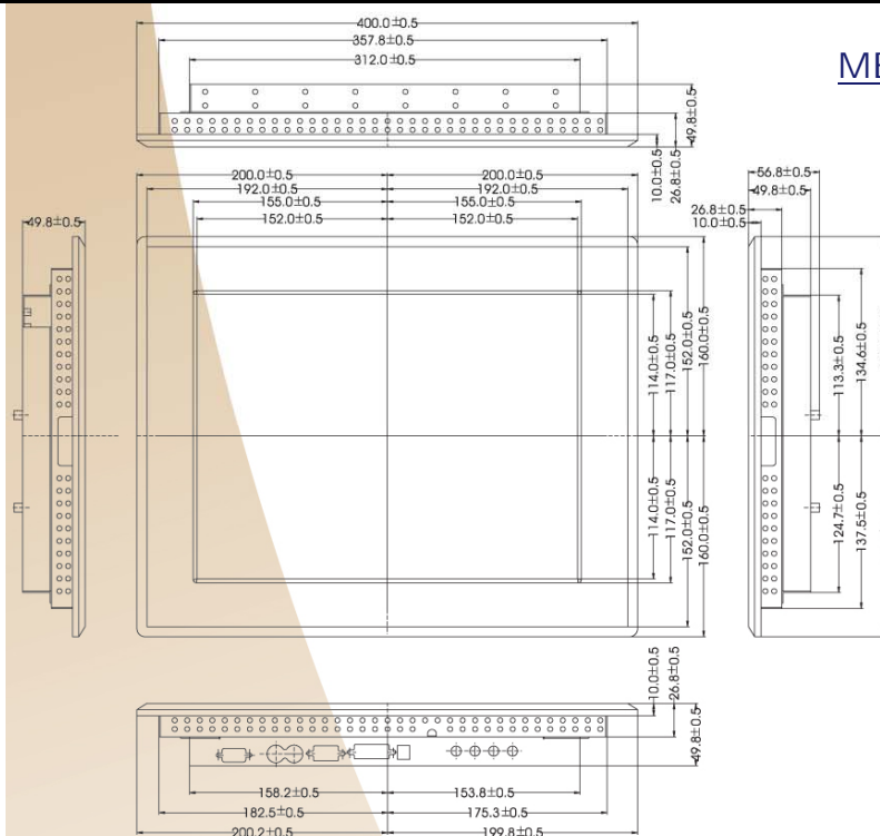
CUT OUT DIMENSION(360x280mm)
