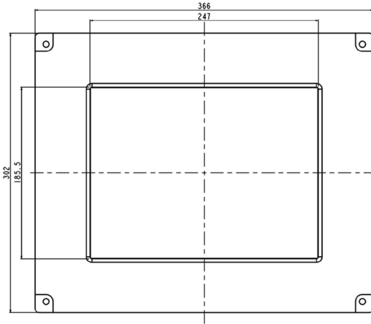
TOP VIEW
