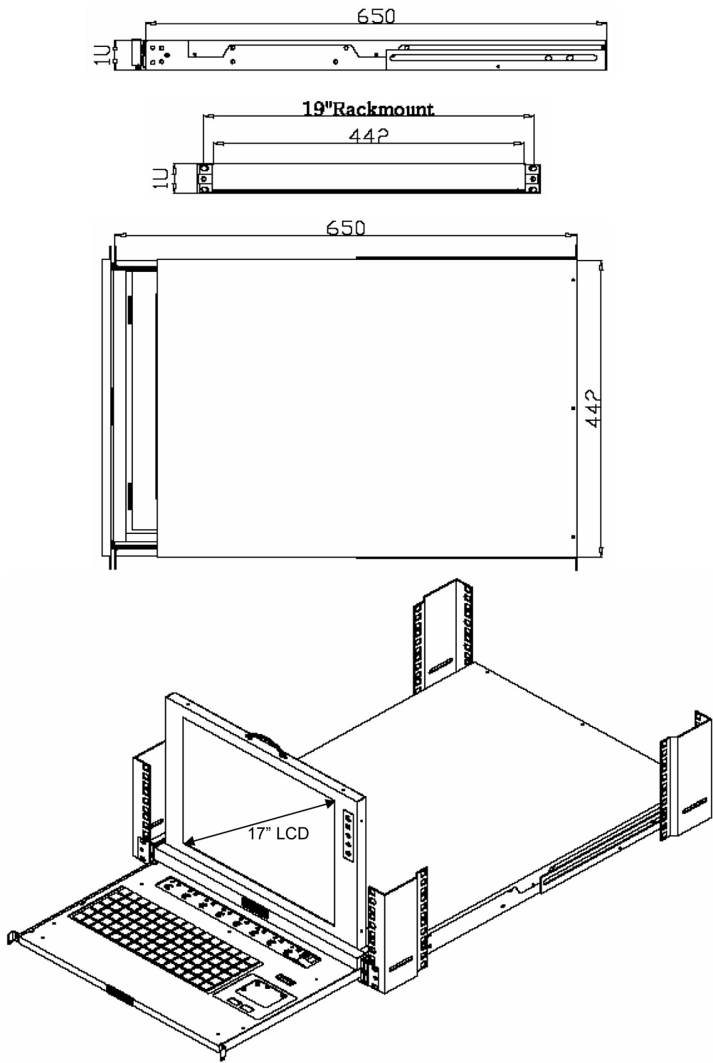
NVP1017-S8/1601 1U 17" LCD Keyboard Drawer with USB KVM
