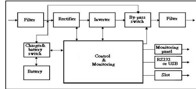
Fig.1. Block diagram
