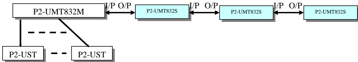
Figure 58 Stacking - Single Base Configuration with P2-UMT832M and P2-UMT832S
