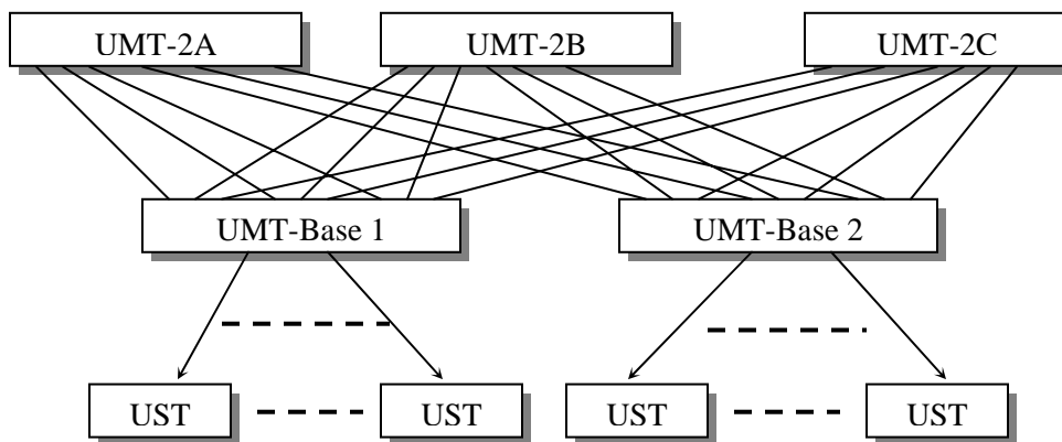
Figure 68 Recommended Redundant Configuration connection scheme
