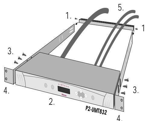
Figure 71 Front rackmount of a P2 Base Unit
