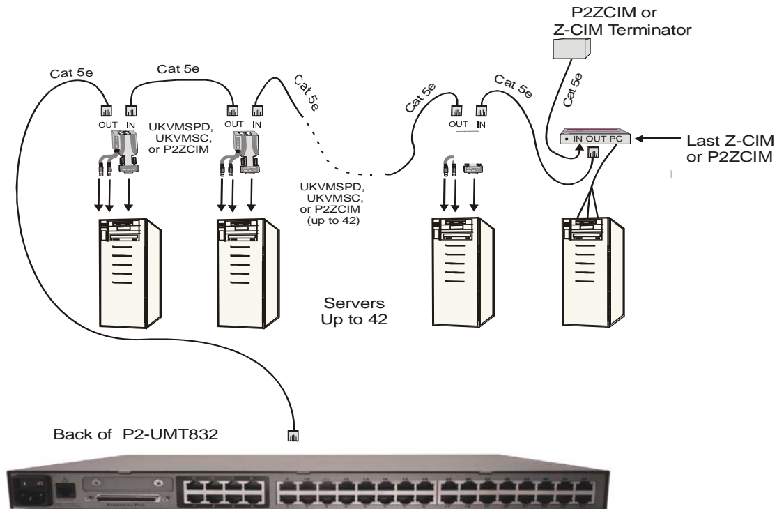
Figure 50 Connecting Z-CIMs or P2ZCIMs as Tiers
