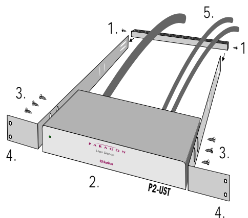
Figure 72 Front rackmount of a P2 User Station
