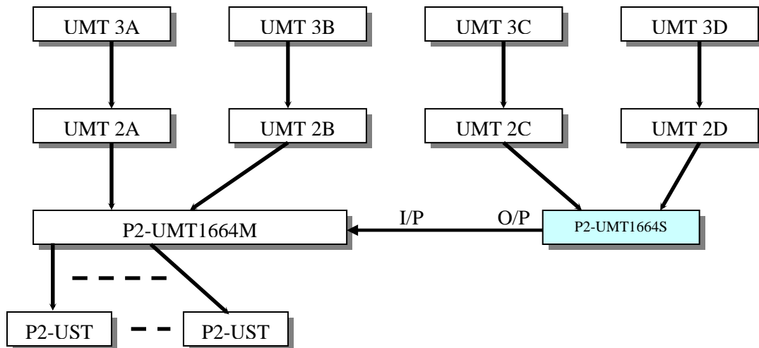
Figure 59 Stacking - Single Base Configuration with P2-UMT1664M and P2-UMT1664S
