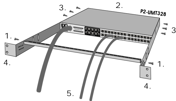
Figure 73 Rear rackmount of a P2 Base Unit
