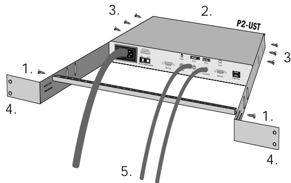
Figure 74 Rear rackmount of a P2 User Station
