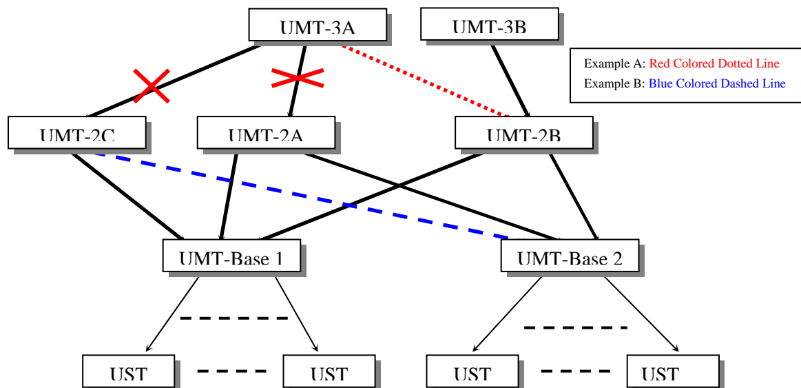
Figure 56 Multiple Base Configuration
