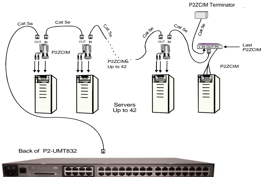
Figure 51 Connecting P2ZCIMs as Tiers to Paragon II
